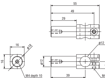
Rotation bracket • φ 12 • 12AL Order code No. 131567 Standard N01864-301L ● Weight : 20.0g
