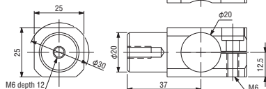
Rotation bracket • φ 20 • 20A Order code No. 131171 Standard N01864-304 ● Weight : 50.7g
