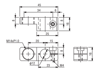
T Connector #1 • \phi 12 \phi 8
