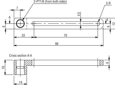
Slide bracket 70 • W • M17
