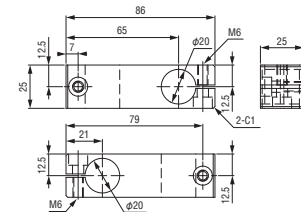
Connector • for SSW
