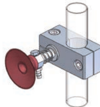
Suction module for jungle gym (φ20)
