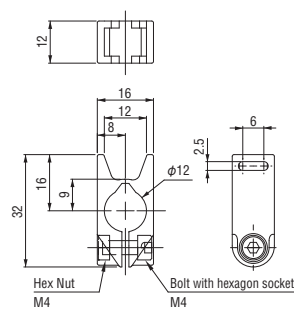
Tie wrap base \phi 12 (tie band)
