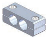
Parallel connector • φ12 φ12 Order code No. 131093 Standard N01861-102 ● Weight : 18.6g
