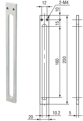
D Vertical bar
