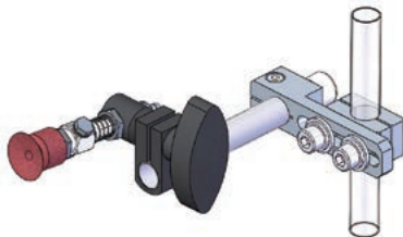
Suction module for jungle gym (φ12)
