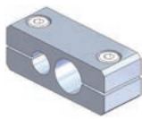
Parallel connector • φ8 φ12 Order code No. 131092 Standard N01861-101 ● Weight : 20.6g
