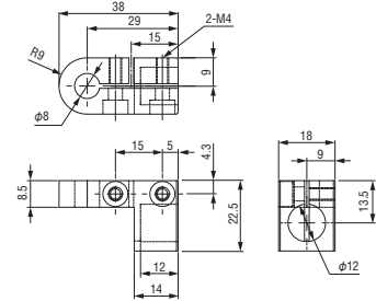
Rotation bracket • φ 12 • 12B Order code No. 131605 Standard N01864-102A ● Weight : 20.0g
