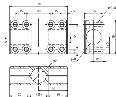
Cross connector # 2 • φ20 φ20 Order code No. 131117 Standard N01861-501 ● Weight : 132.3g
