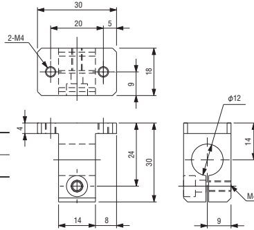
Chuck bracket • φ12
