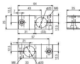
Cross connector • \phi 20 \phi 20 (rear entrance)
