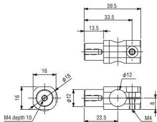
Rotation bracket • φ 12 • 12A Order code No. 131168 Standard N01864-301 ● Weight : 14.6g
