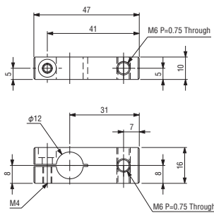
Cylinder bracket • φ 12
