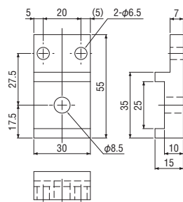
E Sliding chuck fastening bolt
