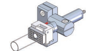
Gripper module • for jungle gym (φ 12)
