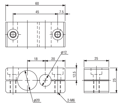
Parallel connector • φ20 φ12 Order code No. 131094 Standard N01861-104 ● Weight : 67.2g
