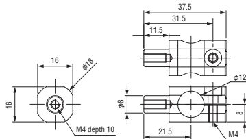
Rotation bracket • φ 12 • 8A Order code No. 131169 Standard N01864-302 ● Weight : 11.9g
