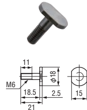
E Sliding chuck fastening bolt
