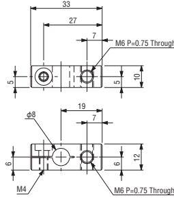
Suction bracket • φ 12 • PT1/8
