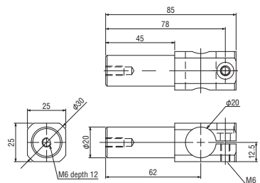
Rotation bracket • φ 20 • 20AL Order code No. 131568 Standard N01864-304L ● Weight : 80.0g
