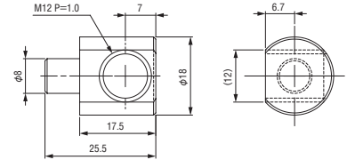
Rotation bracket • φ 12 • 8B Order code No. 131600 Standard N01864-101A ● Weight : 20.6g
