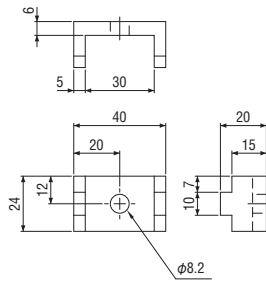
E Sliding chuck fastening bolt H
