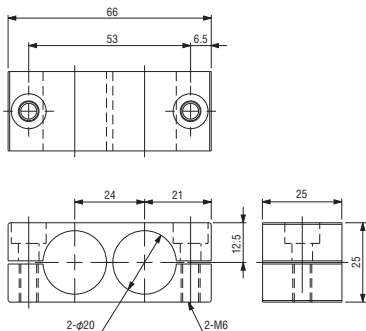
Parallel connector • φ20 φ20 Order code No. 131095 Standard N01861-106 ● Weight : 60.7g
