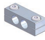
Parallel connector • φ8 φ8 Order code No. 131096 Standard N01861-107 ● Weight : 9.1g
