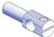
Rotation bracket • φ 12 • 12AL Order code No. 131567 Standard N01864-301L ● Weight : 20.0g
