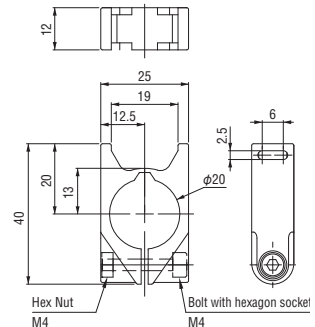
Tie wrap base \phi 20 (tie band)
