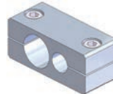
Parallel connector • φ20 φ12 Order code No. 131094 Standard N01861-104 ● Weight : 67.2g
