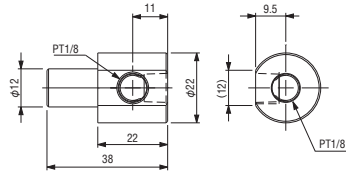
Rotation bracket • φ 12 • PT1/8A Order code No. 131166 Standard N01864-204 ● Weight : 24.6g
