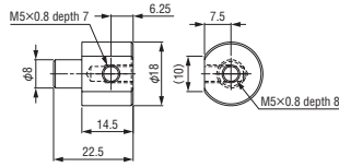
Rotation bracket • φ 8 • M5A Order code No. 131164 Standard N01864-202 ● Weight : 10.0g
