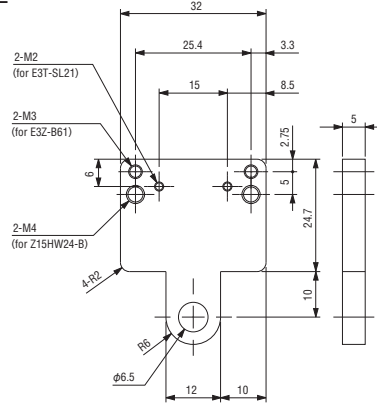
Sensor Mounting Example ②
