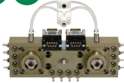
Tool changer • robot side (Load capacity 15kg)
