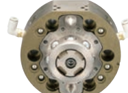
Tool changer for articulated robots • robot side (Load capacity 35kg)
